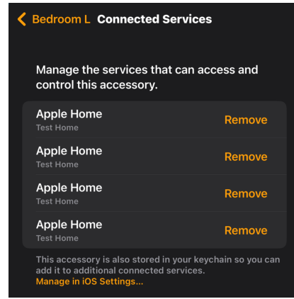
Fig. 5. The owner is entirely incapable of discerning which is his own Apple Home and which belongs to the attacker.
