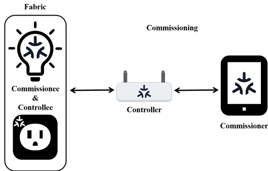
Fig. 1. The Node-Role overview illustrates the interconnections between different node roles within Matter network.
